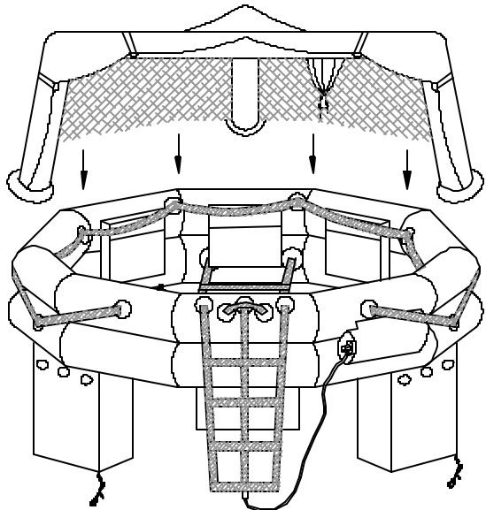
NOT TO SCALE LifeRaft shown with Optional Equipment (Including Optional Canopy)
